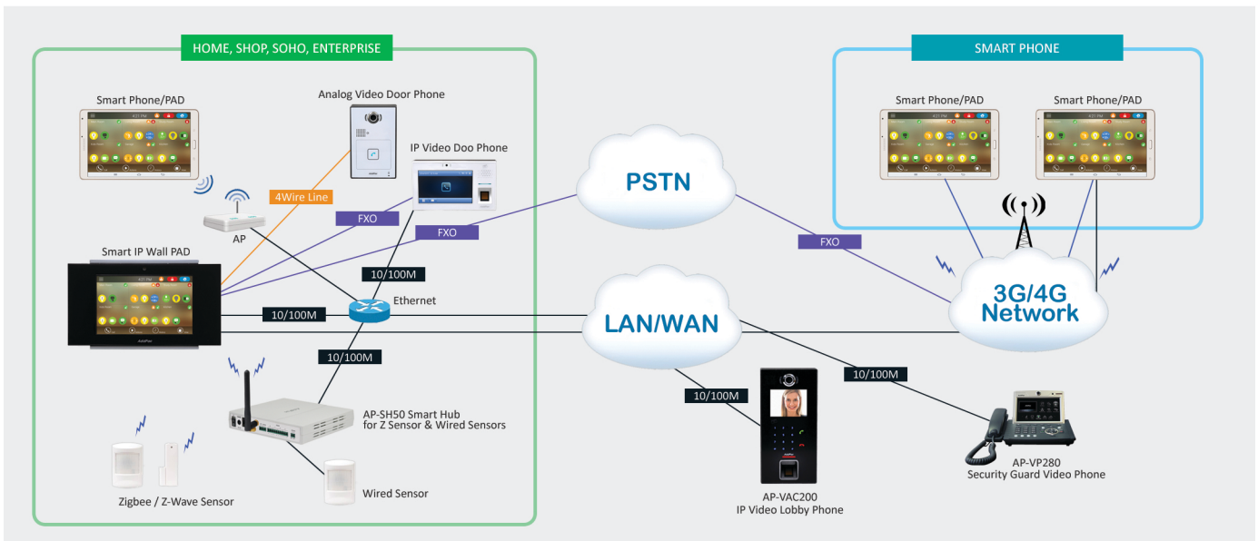
AP-VP280 / AP-VP120 Bidirectional two-way video
